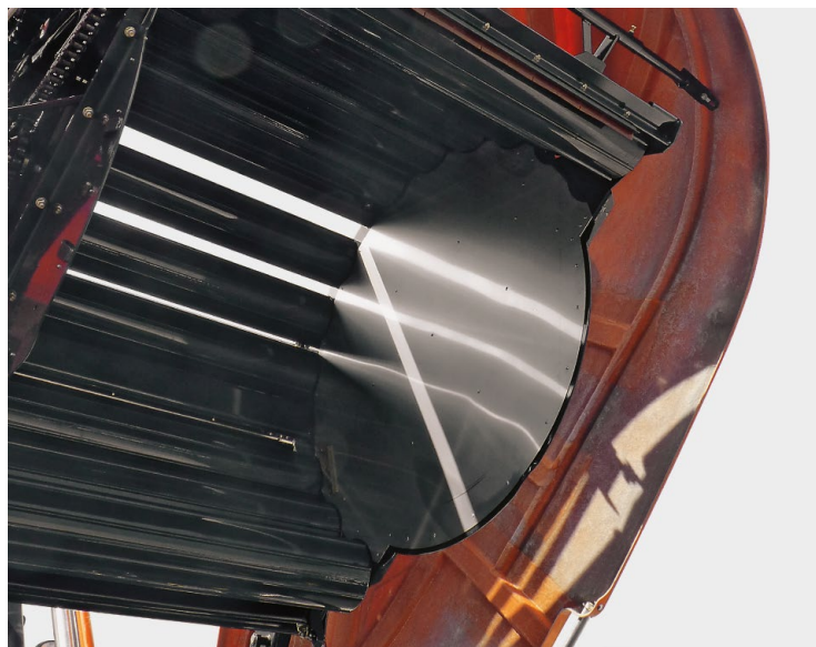
Stainless steel low friction plates
