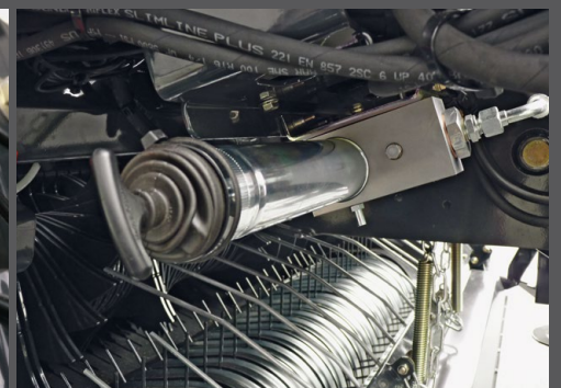
Beka Max automatic bearing greasing system (optional)
